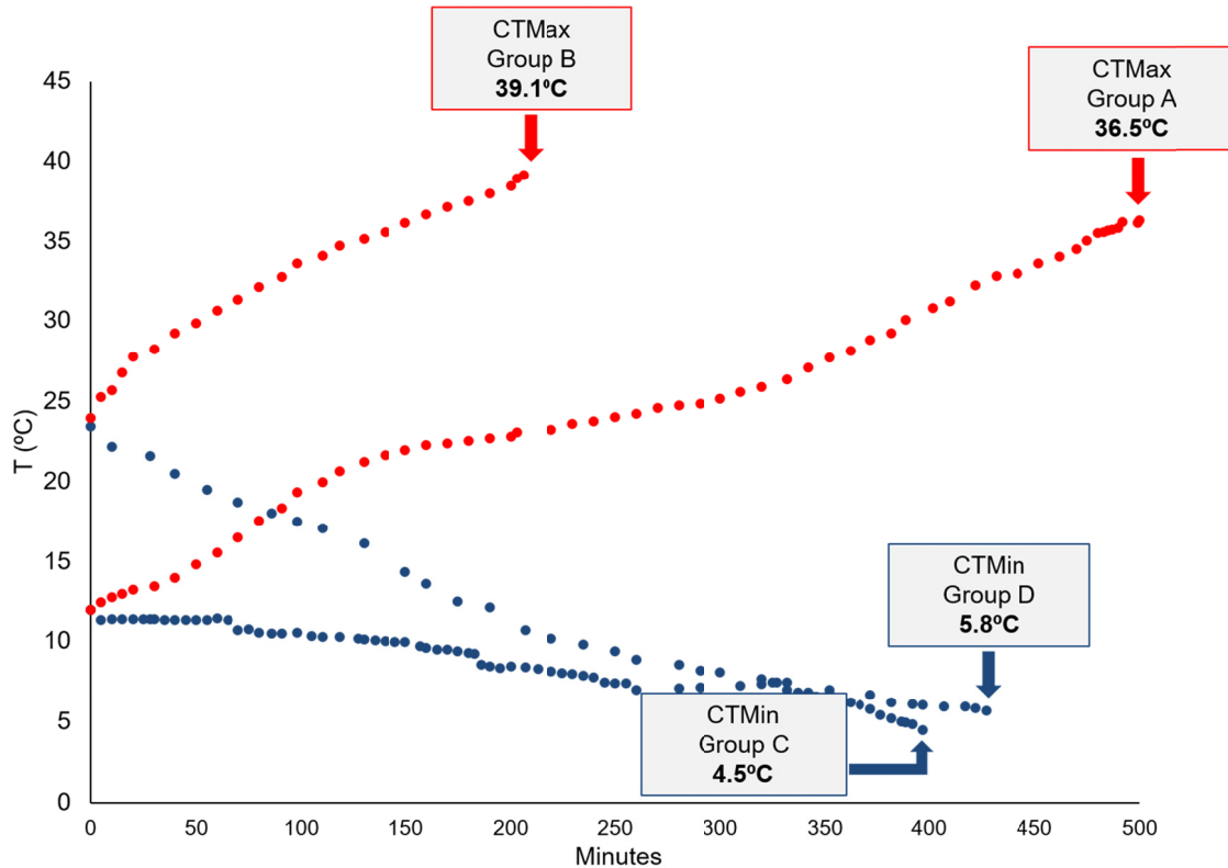
FIGURE 1. CT_{max} and CT_{min} of Australoheros facetus acclimated to different temperatures. In red groups that were heated: Group A from 12°C and Group B from 24°C. In blue groups that were cooled: Group C from 12°C and Group D from 24°C.
